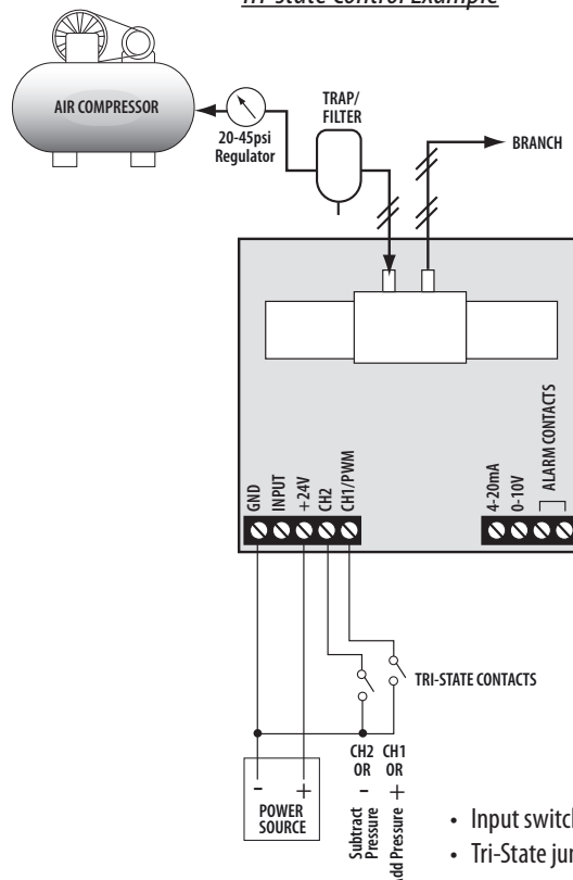
Tri-state Control Example
