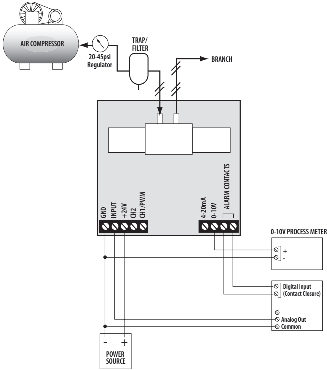
Current/Voltage Control, Voltage Output Example
