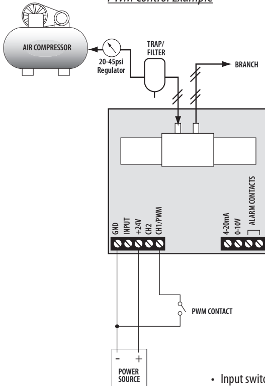
PWM Control Example
